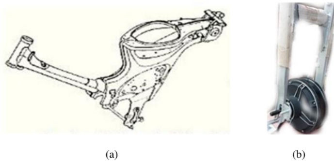
FIGURE 1. The pressed steel frame used in the C-70 motorcycle (a), BLDC motor fitting on the swing arm (b)
