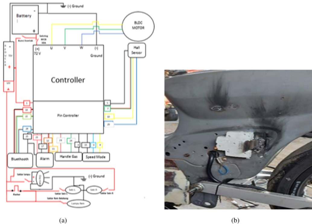
FIGURE 3. Controller on the C-70 electric motorcycle (a), circuit safety system with MCB (b)
