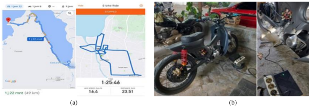
FIGURE 8. The Route Testing at outside and inside Town (a), the battery charging of the C-70 motorcycle (b)
