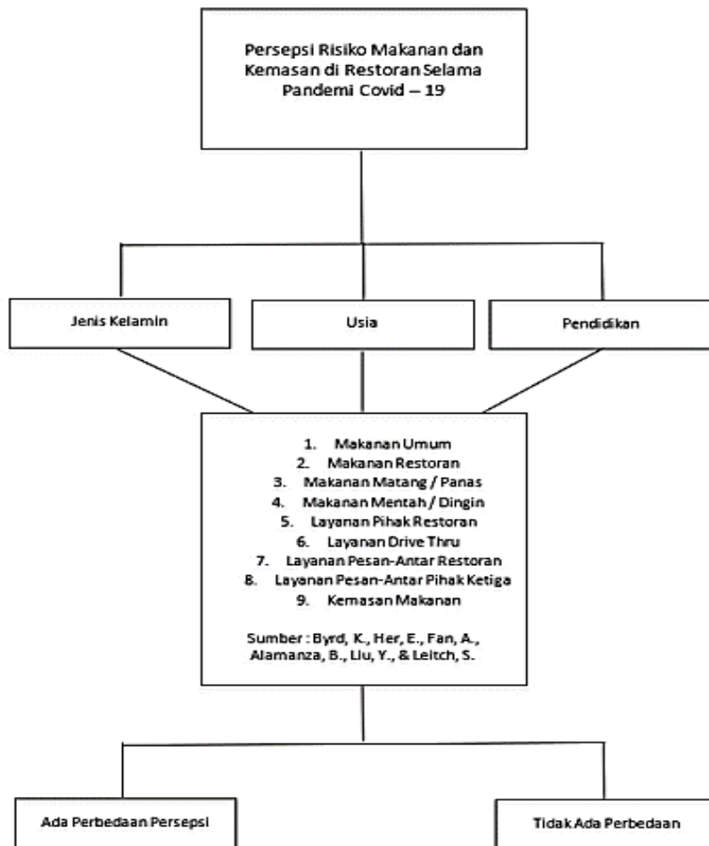
Gambar 1. Model Konseptual
