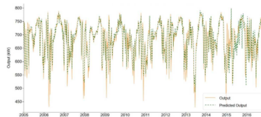
Fig. 4. PV weekly average output vs forecasted results of ARIMAX model (15, 0, 16) for Wonogiri Regency.
