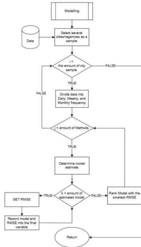
Fig. 1. Modelling flowchart.
