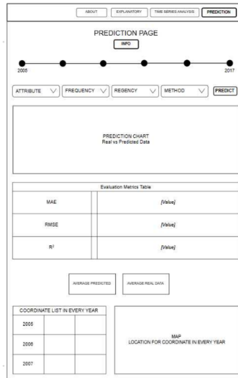
Fig. 2. Visualisation design of the prediction page.
