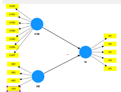
Figure 2. Path Diagram
