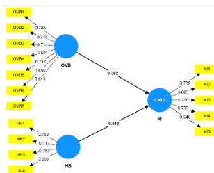
Figure 3. Path Diagram
