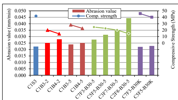
Fig. 6. Abrasion resistance of selected samples and their 28-day compressive strength.
