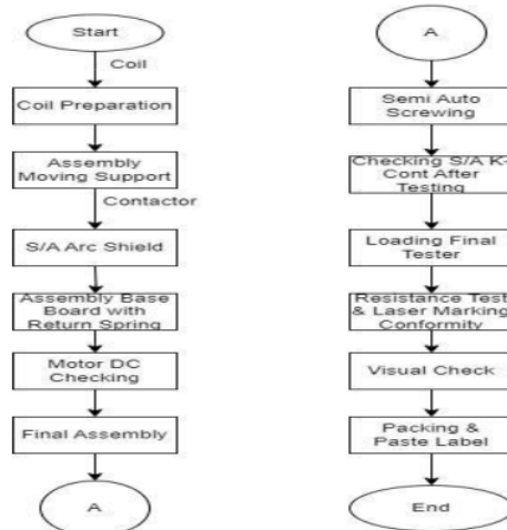
Fig 1. K-Contactor's backend production process
