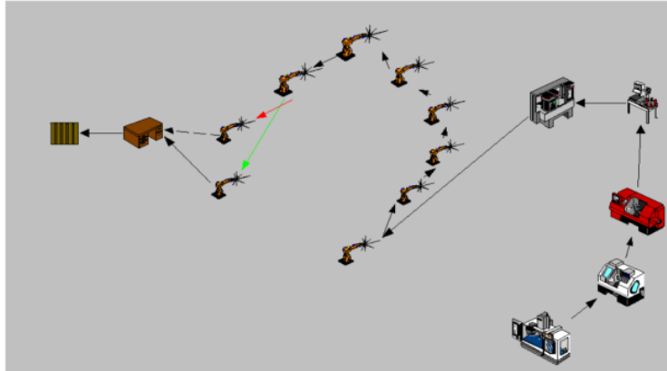
Fig. 2. Initial Layout Model.
