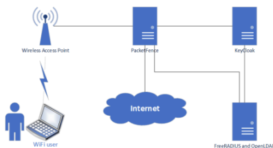
Figure 1. Implementation Design
