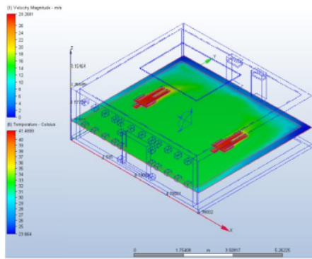
Figure 15 Temperature Planes by CFD Source: Author, 2023
