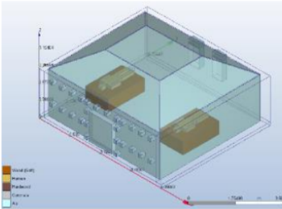
Figure 10 CFD Model Source: Author, 2023
