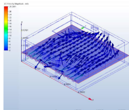
Figure 13 Planes and trace visualization mode by CFD Source: Author, 2023
