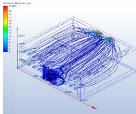
Figure 14 Trace visualization mode by CFD Source: Author, 2023
