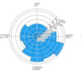
Figure 9 Wind Frequency Rose (GWA, 2023)
