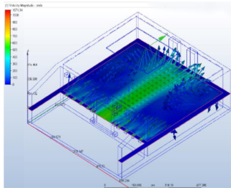
Figure 15 Planes visualization mode by CFD Source: Author, 2023)
