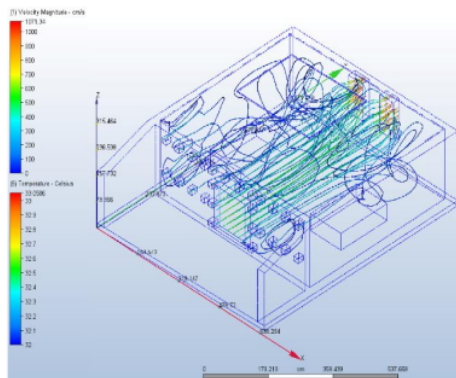
Figure 16 Trace visualization mode by CFD Source: Author, 2023)
