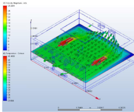
Figure 16 Temperature Planes w Velocity Vector by CFD Source: Author, 2023
