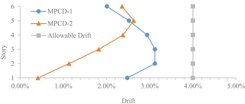
Fig. 5. Story drift.
