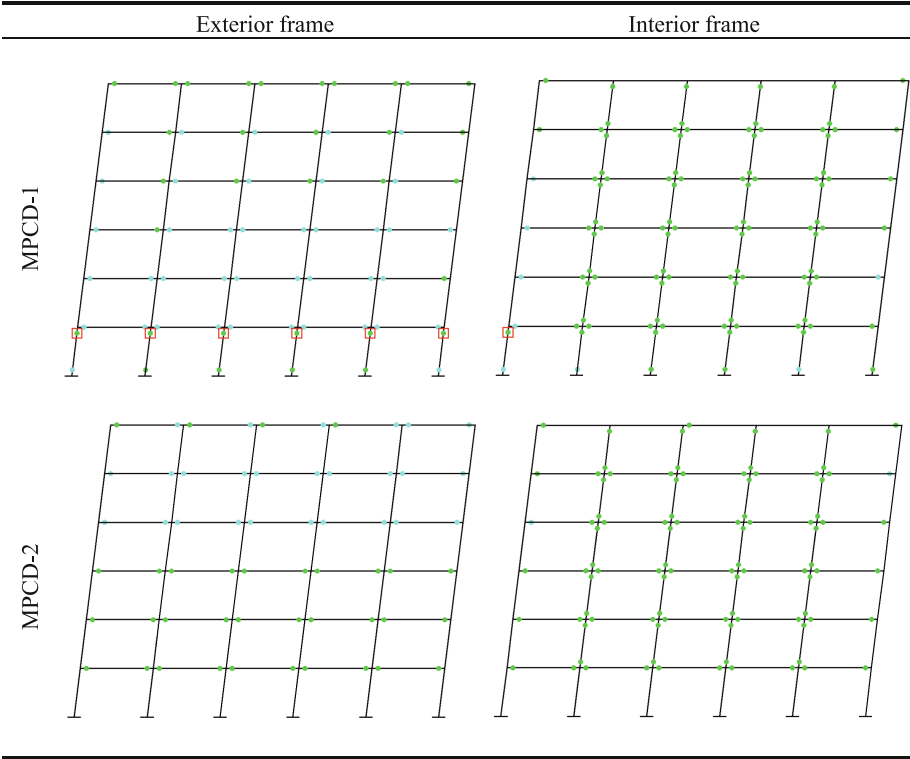
Fig. 3. Plastic hinge configuration.
