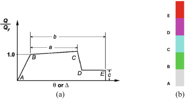
Fig. 4. Hinge state: (a) generalized force-displacement relation [10] (b) color indicator.
