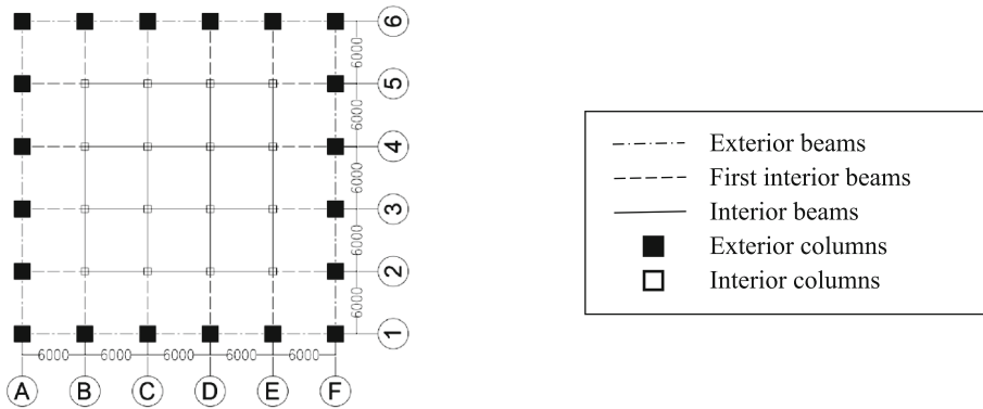
Fig. 2. Typical floor plan.
