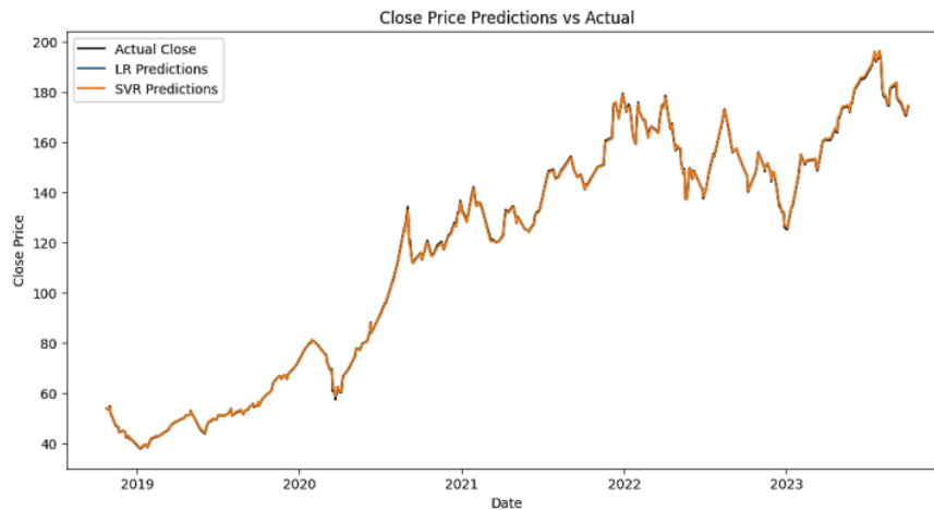
Figure 3. Model comparison chart
