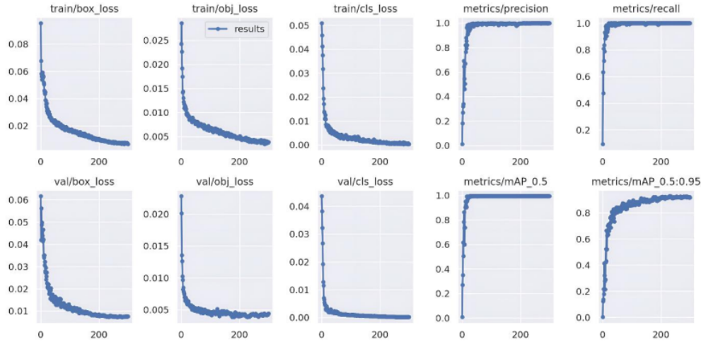
Fig. 6. Training result graph.
