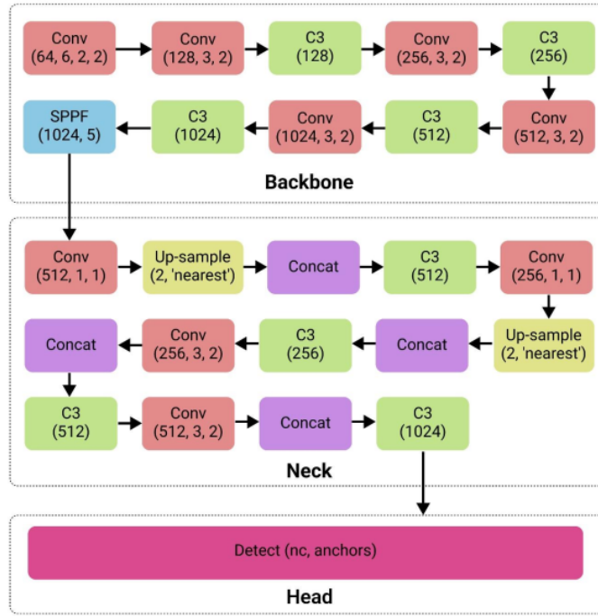
Fig. 5. The YOLOv5m architecture adapted from [21].
