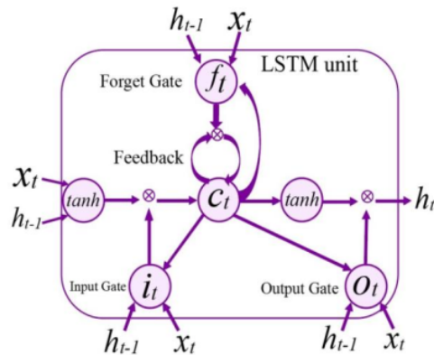
Figure. 1 One Memory Cell of LSTM Unit
