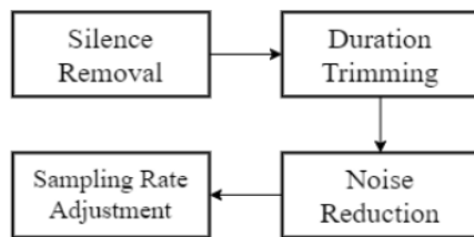
Figure. 3 Speech Data Preprocessing Steps
