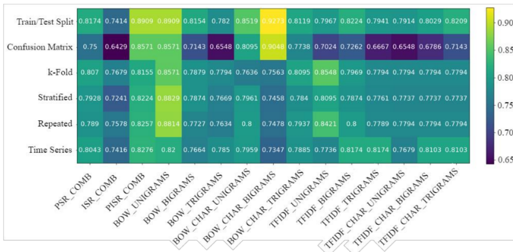
Figure. 12 Graphical Heatmap Result of Train/Test Split, Confusion Matrix, k-Fold, and Cross-Validation (k=5) methods
