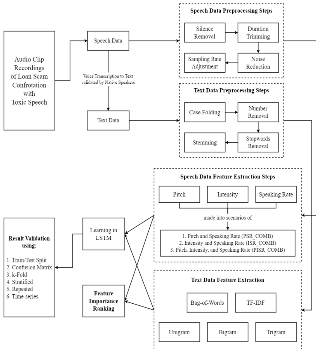
Figure. 2 Proposed Experiment Pipeline
