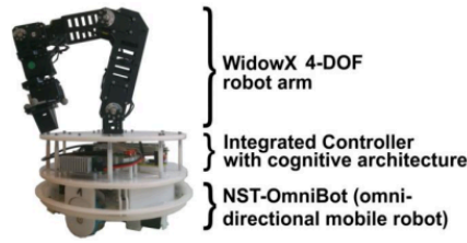
Figure 7. The mobile manipulator developed for the test case of our model-based learning method. It is composed of two subsystems: a 4-DOFs robotic arm and a mobile platform.
