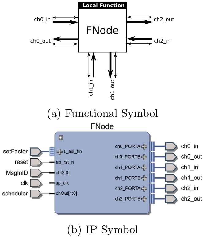
Fig. 6. FNode symbol representation.
