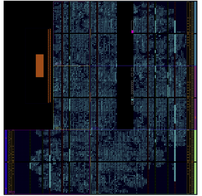
Fig. 14. Floorplan view of the design without optimization for the network shown in Fig. 11. This was implemented on SoC XC7Z020, and we used cardinality value of five for the network.
