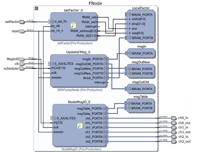
Fig. 7. Internal block diagram of module FNode shown in Fig. 6b.
