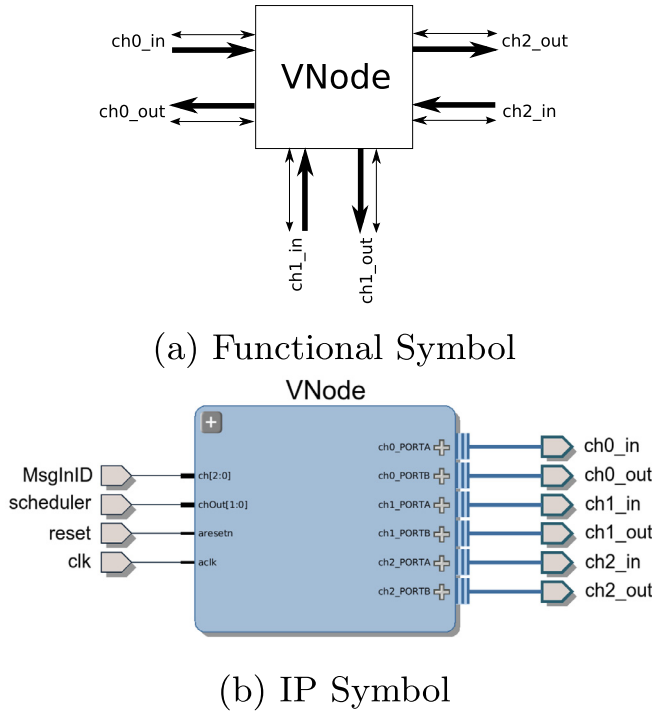
Fig. 8. VNode symbol representation.
