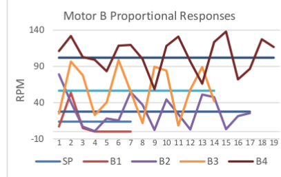
Figure 9. Motor B Poropotional responses
