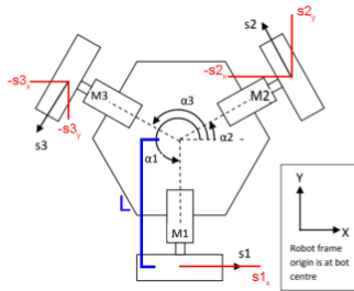
Figure 3. Odometry calculation
