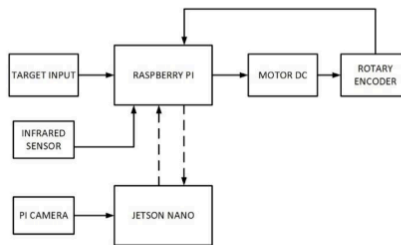
Figure 1. Block diagram of an omni-directional robot system
