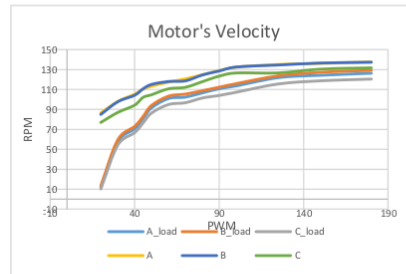
Figure 7. Motor's velocity readings with encoder.
