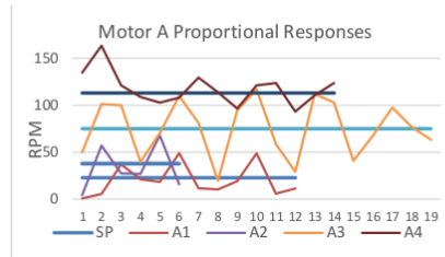
Figure 8. Motor A Poropotional responses
