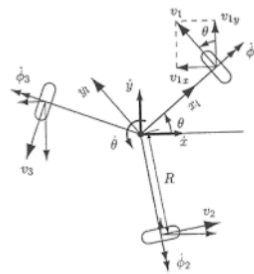
Figure 2. Three wheeled robot's kinematics
