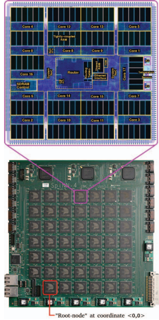
Fig. 1. 48-node SpiNNaker board. Each chip contains 18 ARM968 cores (shown on top figure) and 128MB SDRAM mounted on top of the processor die. A special chip labeled as “root-node” contains an RTM supervisor that coordinates all other RTMs in each chip on the board.
