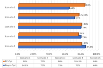
Fig. 5. Optimized BiLSTM-CNN Accuracy Result
