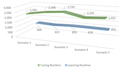
Fig. 4. BiLSTM-CNN Runtimes optimized by Bayes-Opt (in seconds)
