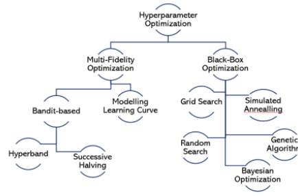
Fig. 1. A classification of hyperparameter optimization methods [12]
