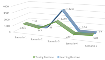
Fig. 3. BiLSTM-CNN Runtimes optimized by RF-Opt (in seconds)
