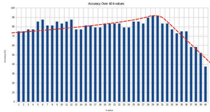
Fig. 7 Achieved accuracy for each possible k-values in the range of 40 k-values. This also corresponds to the distributed k-value across worker cores
