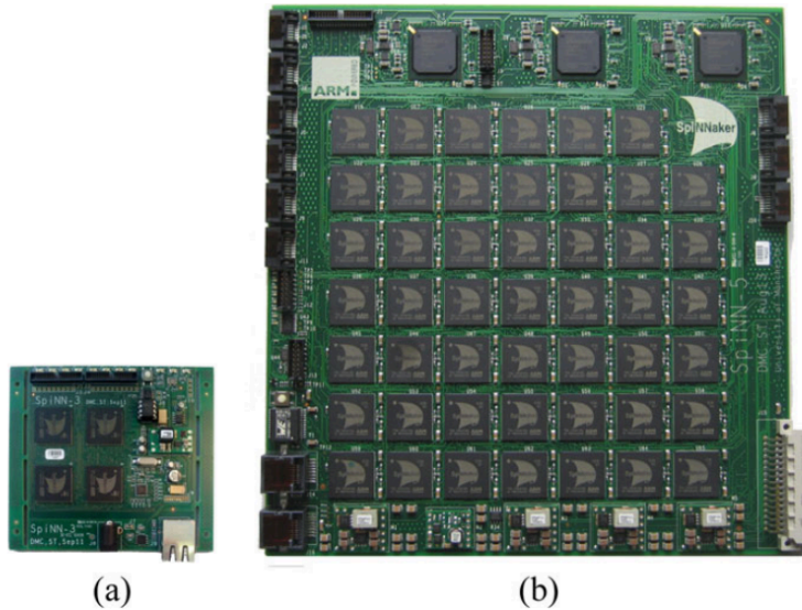
Fig. 1 Two types of SpiNNaker boards: a Spin3 with 4 SpiNNaker chips, and b Spin5 with 48 SpiNNaker chips
