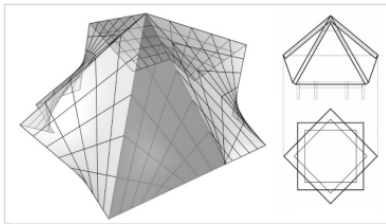
Figure 8. Initial roof geometry
