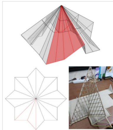
Figure 13. Third alternative: Geometry and scaled model
