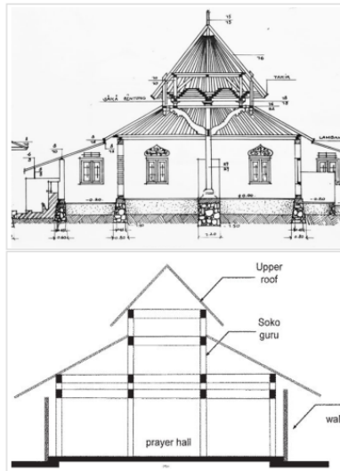
Figure 3. Example of saka tunggal (top) and saka guru (bottom) cross-section in Indonesian traditional Mosque (Bambang Setia Budi 2006; Wibowo and Sasano 2016)
