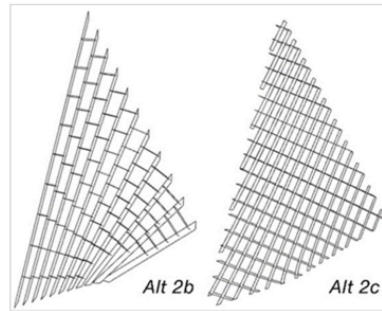
Figure 9. Roof construction alternatives 1 and 2a-c
