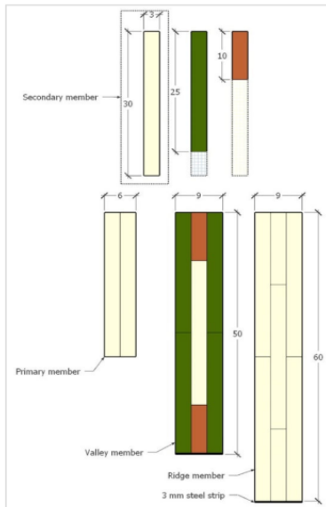
Figure 14. Timber member sections
