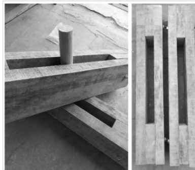
Figure 12. Alternative 2d joints prototype
