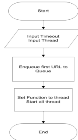
Figure 3.2 main threading process
