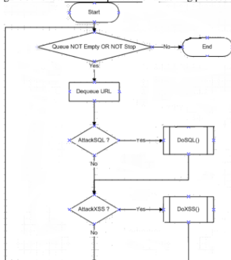
Figure 3.4 attacking process main flowchart
