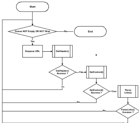
Figure 3.3 main flowchart crawling process
