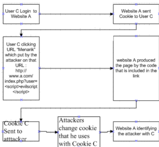
Figure 2.3 flowchart of request / response match method
