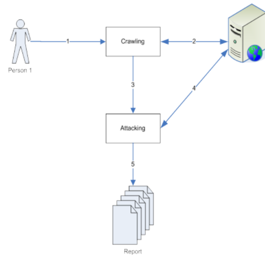
Figure 3.1 main system flowchart
