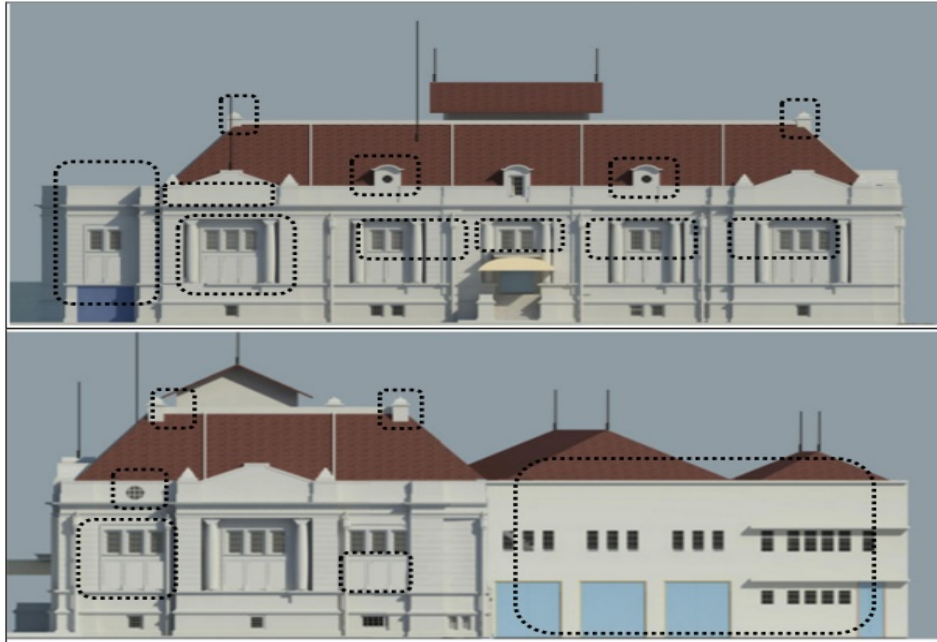
Figure 3. the existing condition of the north elevation (top), and the west elevation in 2009 (bottom)
