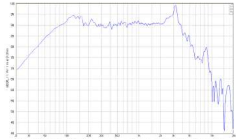
Gambar 9. Spektrum Analyzer Middle Speaker
