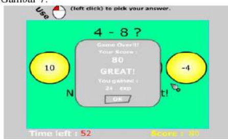
Gambar 6. Score Window
