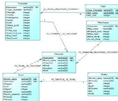
Gambar 2. ERD System
