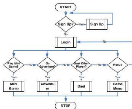
Gambar 1. Flowchart System
