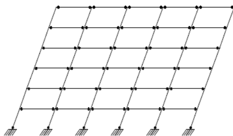
Figure 1. Sidesway Mechanism
