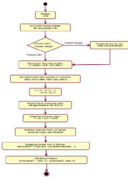
Gambar 2. Flowchart Forecasting
