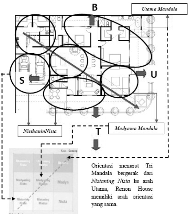
Gambar 9. Analisis Arah Hadap dan Orientasi Renon House.
