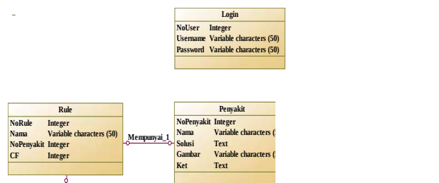
Gambar 3 Conceptual ERD
