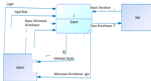
Gambar 2 Context Diagram
