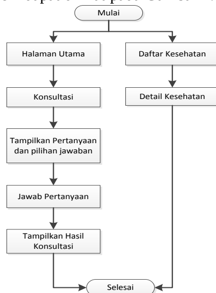
Gambar 1 Flowchart Sistem
