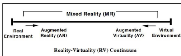
Fig. 1 Mixed Reality [13]
