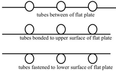
Figure 2. Tube arrangement and the plate absorber
