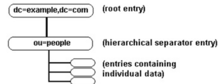
Fig. 1. DIT (Directory Information Tree) structure
