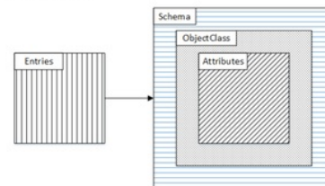
Fig. 2. LDAP Schema Structure
