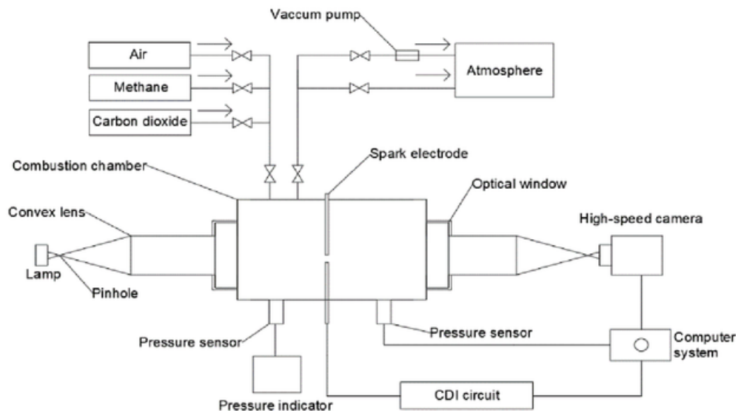
1 Fig. 1. Schematic of experimental setup.
