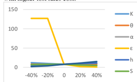
Figure 2. The sensitivity analysis for the optimal price
