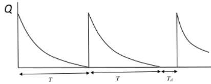
Figure 2. Inventory level in the last harvest period
