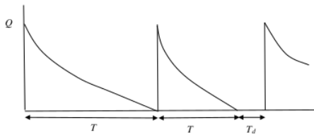
Figure 1. Inventory level for preliminary harvest period
