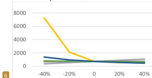
Figure 4. The sensitivity analysis for optimal total profit
