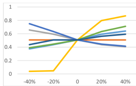
Figure 3. The sensitivity analysis for optimal replenishment time
