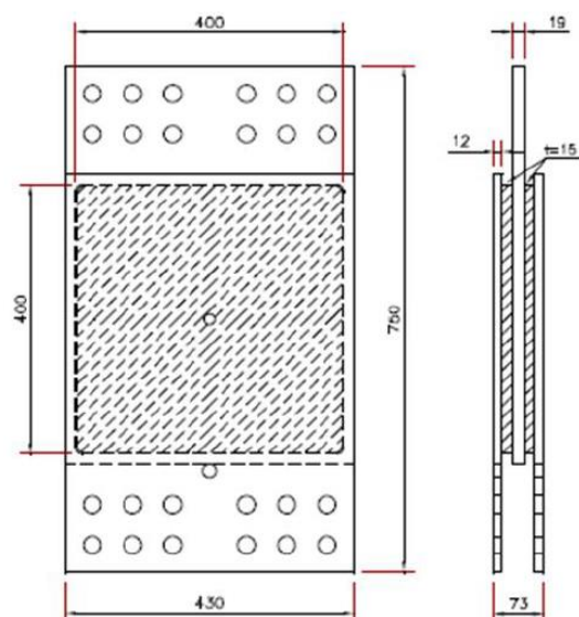
Figure 1. VSL-Gensui Damper
