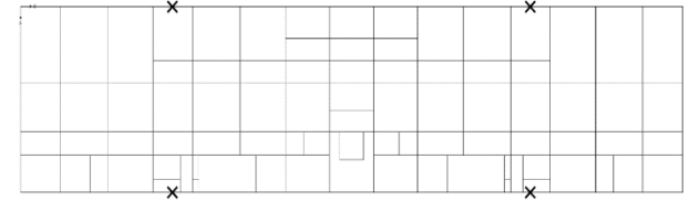
Figure 13. Damper Placement at 4 th floor (R-X and SR-X); MSSSA: 0 damper; ODAM: 4 dampers
