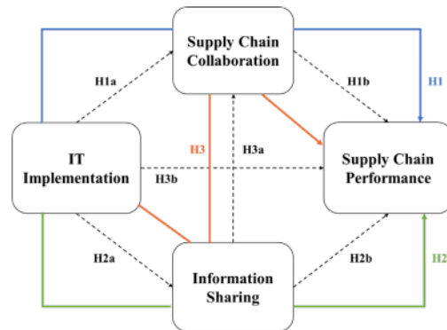
Figure 1. Research framework
