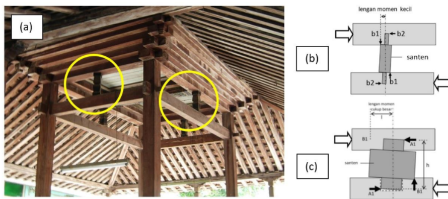
Fig. 4: (a) The position of santen on the core structure ( rong-rongan ) of the joglo building, (b) original santen , (c) santen with extended torque arm to withstand the lateral shear forces. Source: Maer, 2015
