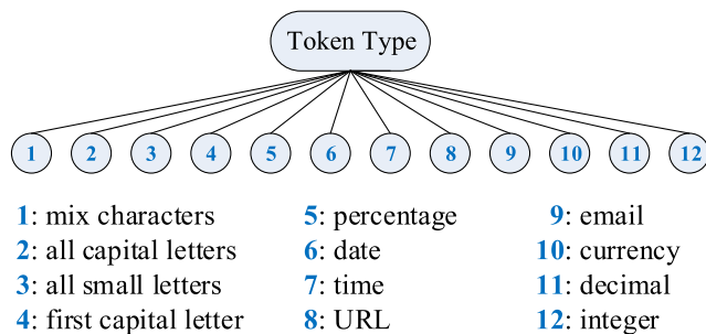
Fig. 4 Token types
