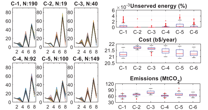
Fig. 12. (left) Six capacity clusters (y-axis = GW of capacity for each available generation option along the x-axis) and (right) unserved energy, cost and CO 2 emissions of all clusters CP60.
