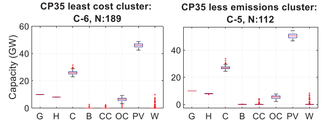
Fig. 11. (left) Technology mixes in the least cost cluster (C-6) and (right) technology mixes in the 'lower' emissions cluster (C-5) for 5% least cost portfolios with CP35.
