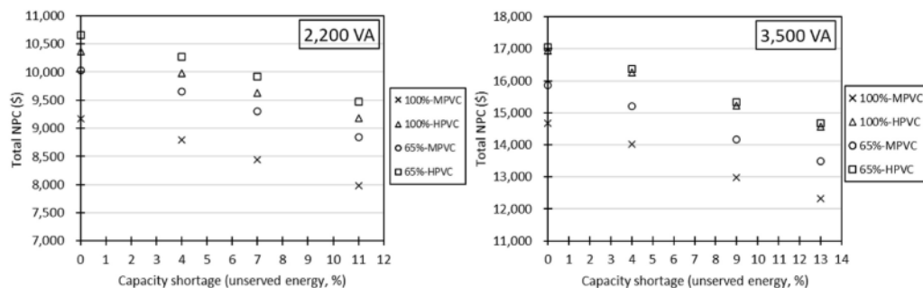
Fig. 5. Total NPC versus unsurved energy in all cases for 2,200 VA (left) and 3,500 VA (right).
