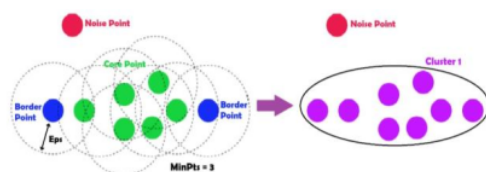
Fig. 4 Example of DBSCAN clustering process with MinPts = 3.
