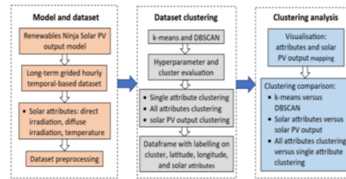
Fig. 2 Framework for assessing solar attributes clustering.
