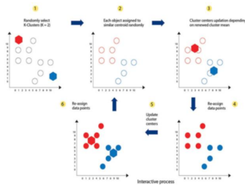
Fig. 3 Example of k-means clustering process with k = 2 .
