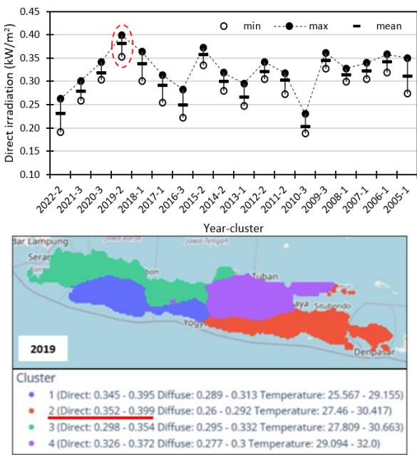
Fig. 6 Clustering results of direct irradiation obtained from the k -means three-attribute clustering: (Top) the years and clusters showing a range of values among clusters with the highest value of yearly average direct irradiation in each year; and (Down) the 2019 Java-Bali's clustering map showing the corresponding area (in Red).
