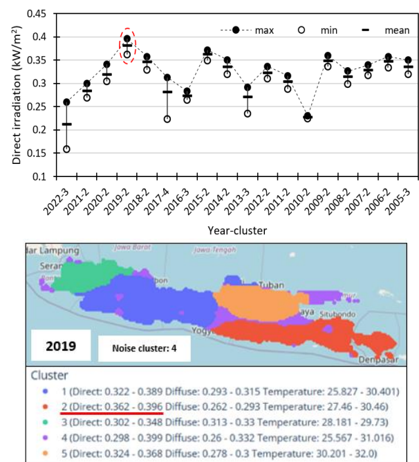
Fig. 16 Clustering results of direct irradiation obtained from the DBSCAN three-attribute clustering: (Top) the years and clusters showing a range of values among clusters with the highest value of yearly average direct irradiation in each year; and (Down) the 2019 Java-Bali's clustering map showing the corresponding area (in red).
