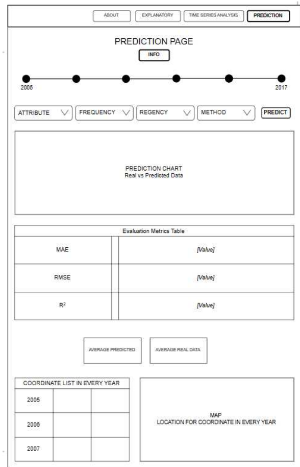
Fig. 2. Visualisation design of the prediction page.
