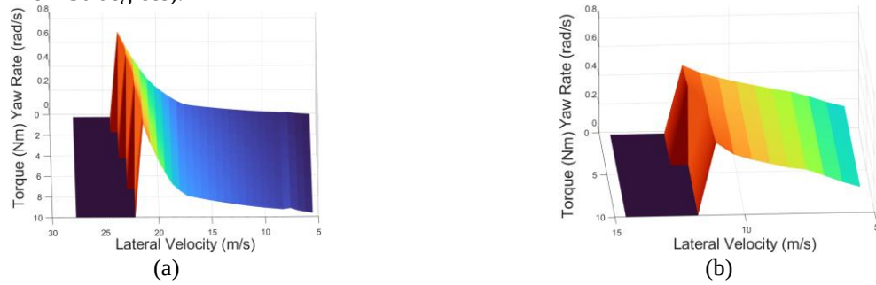
FIGURE 1. Yaw rate response at a constant steering angle (a) 5 degrees and (b) 75 degrees
