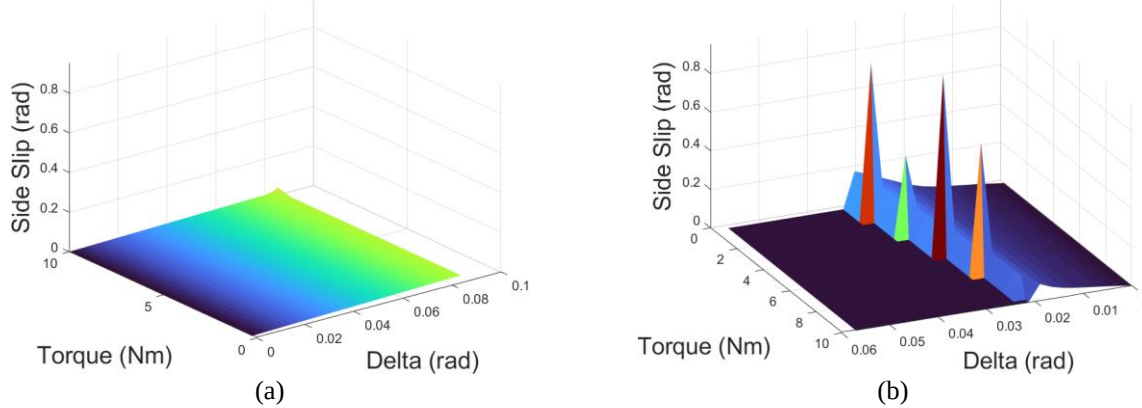
FIGURE 4. Side slip angle response at a constant longitudinal speed (a) 35 km/h and (b) 65 km/h
