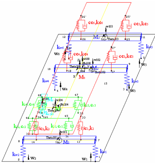
Gambar 1. Model dinamik truk 3 axle [9]
