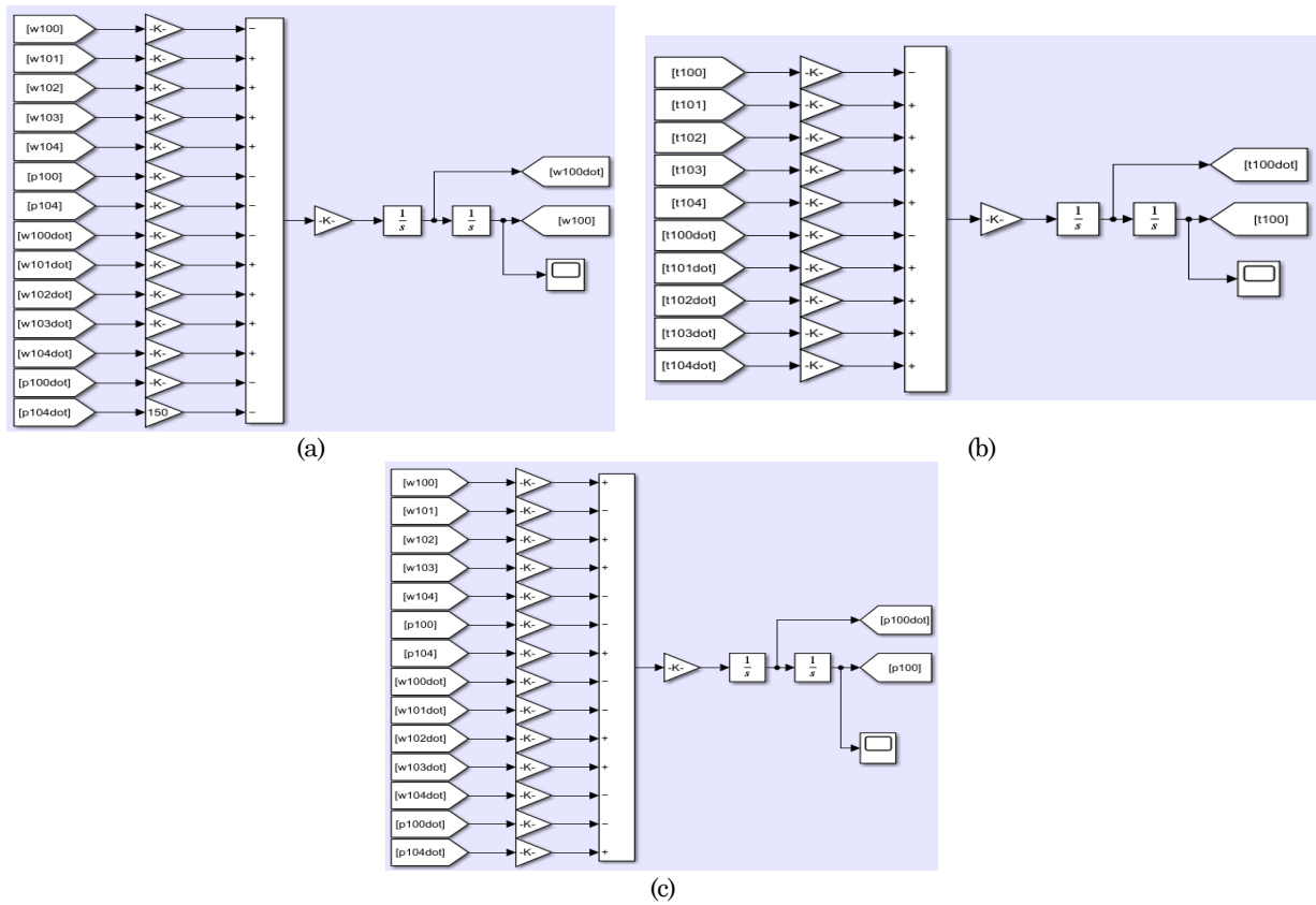
Gambar 2. Block Simulink body truk (a) gerakan vertical, (b) gerakan rolling, (c) gerakan pitching
