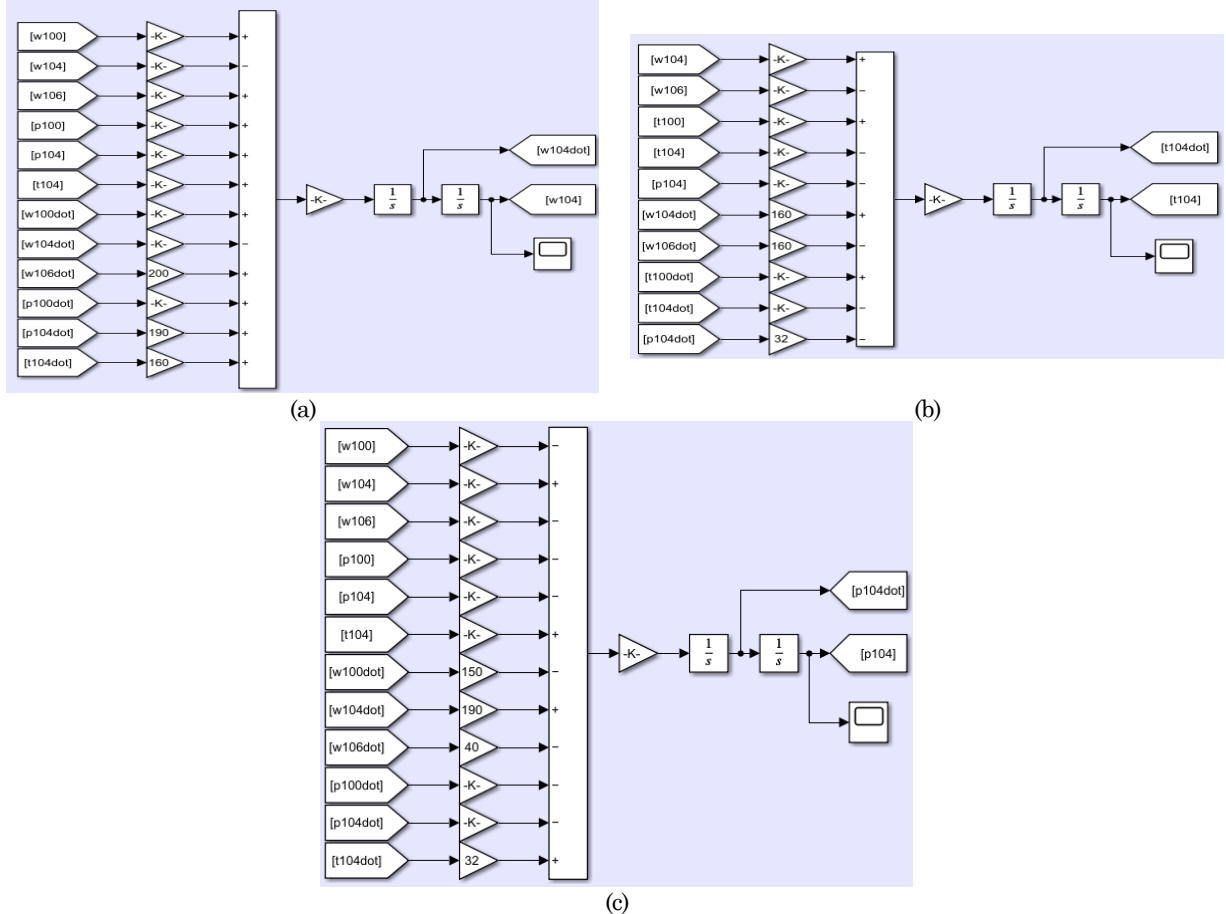
Gambar 3. Block Simulink kepala truk (a) gerakan vertical, (b) gerakan rolling, (c) gerakan pitching
