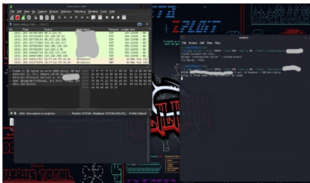
Fig. 8 . TCP Syn Flood Attack Second Results Using Hping3 and Wireshark on Kali Linux
