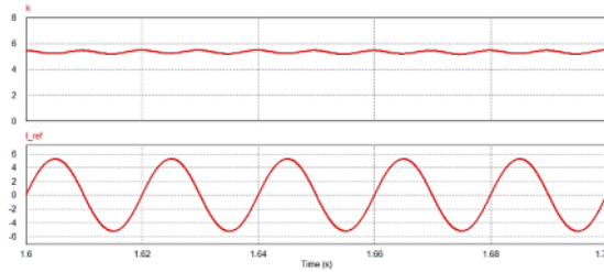
Fig. 18 The PI controller output signal (top) and i_{ref} (bottom) for P_{inv} < P_{load}
