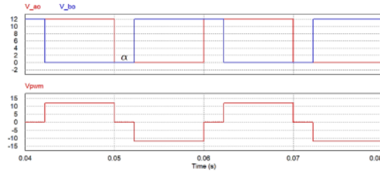
Fig. 4 Three-level square wave with a displacement angle \alpha
