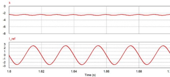
Fig. 15 The PI controller output signal (top) and i_{ref} (bottom) for P_{inv} > P_{load}
