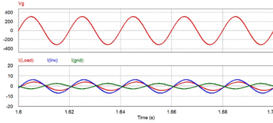
Fig. 13 The grid voltage (top) and the currents of the grid, the VSI, and the load (bottom) for P_{inv} > P_{load}
