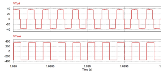
Fig. 8 Transformer primary (top) and secondary (bottom) voltages for \alpha = 29^\circ
