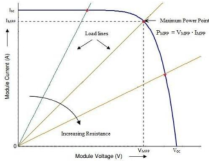
Fig. 5 Load lines of the PV panel [12]
