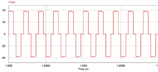
Fig. 10 Transformer primary voltage for \alpha = 60^\circ
