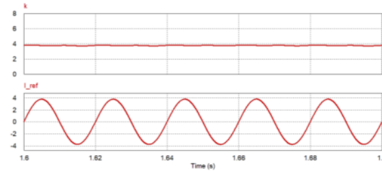
Fig. 18 The PI controller output signal (top) and i_{ref} (bottom) for very low irradiance
