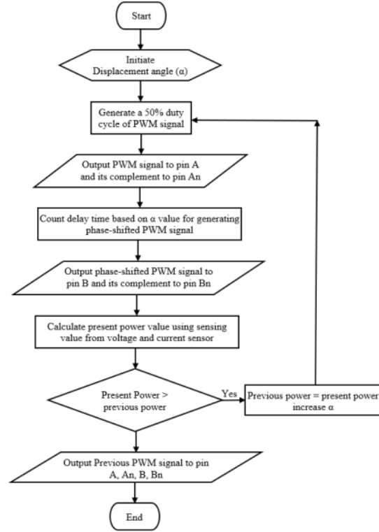
Fig. 3 Simple algorithm for controlling switching time
