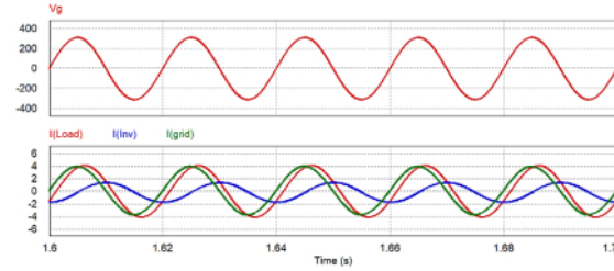
Fig. 20 The grid voltage (top) and the currents of the grid, the VSI, and the load (bottom) for very low irradiance
