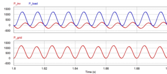
Fig. 21 The VSI power, the load power (top), and the grid power (bottom) for very low irradiance
