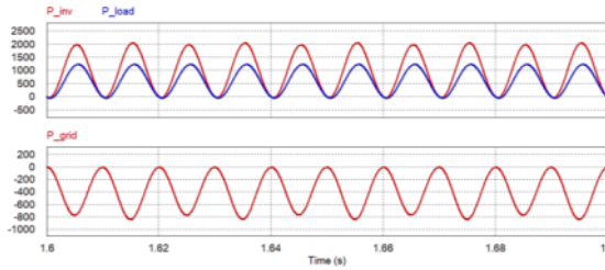
Fig. 14 The VSI power, the load power (top), and the grid power (bottom) for P_{inv} > P_{load}
