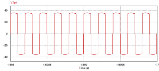
Fig. 12 Transformer primary voltage for \alpha = 10^\circ
