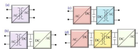
Fig. 1 Configurations of SST a) single stage, b) and c) two stages, d) three stages [6]
