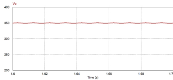
Fig. 6 DC Bus Voltage ( V_o )
