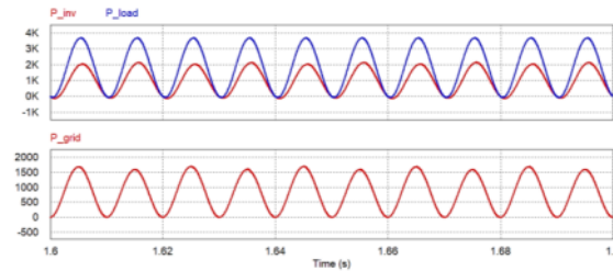
Fig. 17 The VSI power, the load power (top), and the grid power (bottom) for P_{inv} < P_{load}
