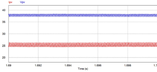
Fig. 9 PV output voltage and current for \alpha = 60^\circ
