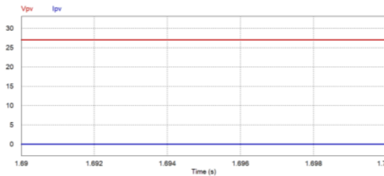
Fig. 19 PV output voltage and current for very low irradiance
