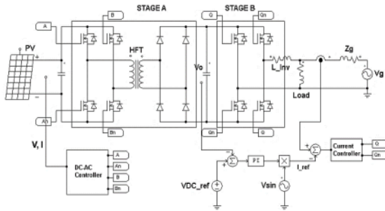
Fig. 2 Diagram of the grid-connected PV system
