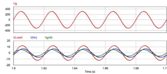
Fig. 16 The grid voltage (top) and the currents of the grid, the VSI, and the load (bottom) for P_{inv} < P_{load}
