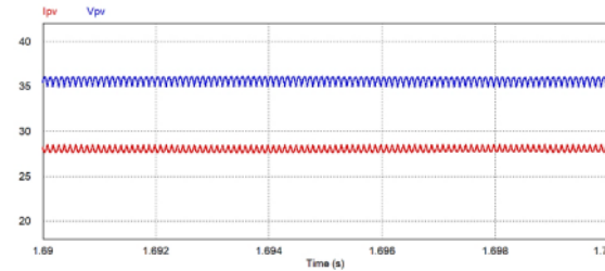
Fig. 7 PV output voltage and current for \alpha = 29^\circ
