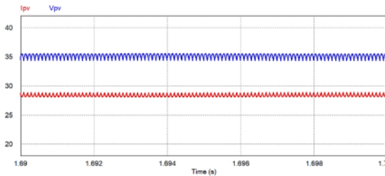
Fig. 11 PV output voltage and current for \alpha = 10^\circ
