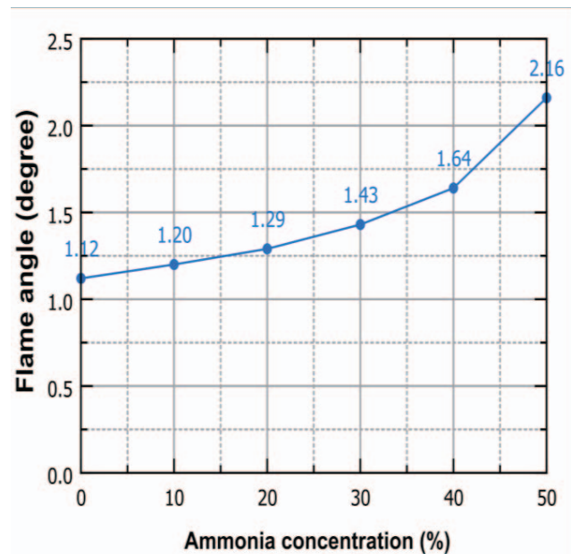
Figure 3. Relationship between ammonia gas content and flame angle.
