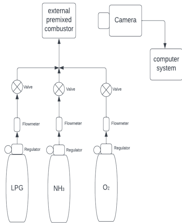
Figure. 1. Schematic diagram of an experimental system
