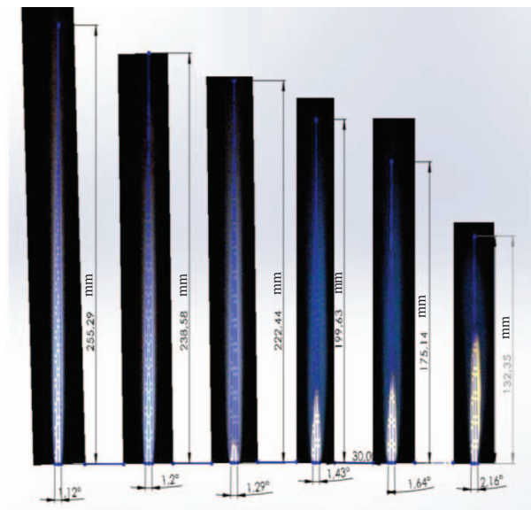
Figure 2. Images of the flame under ammonia addition conditions (0% to 50% from left to right, with 10% increments, respectively)
