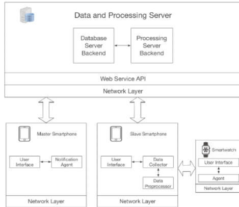
Fig. 6. Mobile sensing platform architecture [7]
