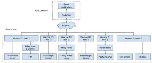
Fig. 5. Block diagram of the smart home [7]
