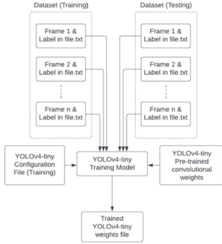
Fig. 3. The block diagram of YOLOv4-tiny training process.
