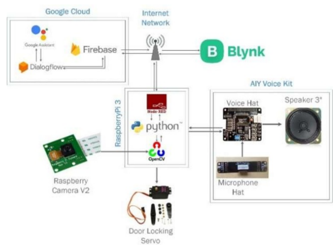
Fig. 3. Block diagram of smart door system [9].
