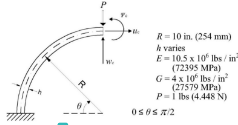
4 Fig. 5. A quarter circular cantilever arch.
